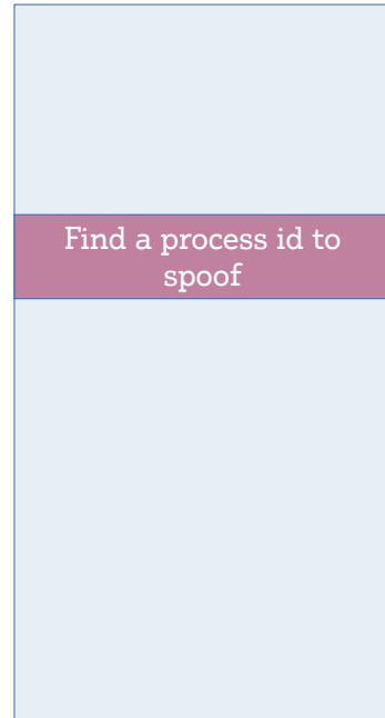
Malware process
